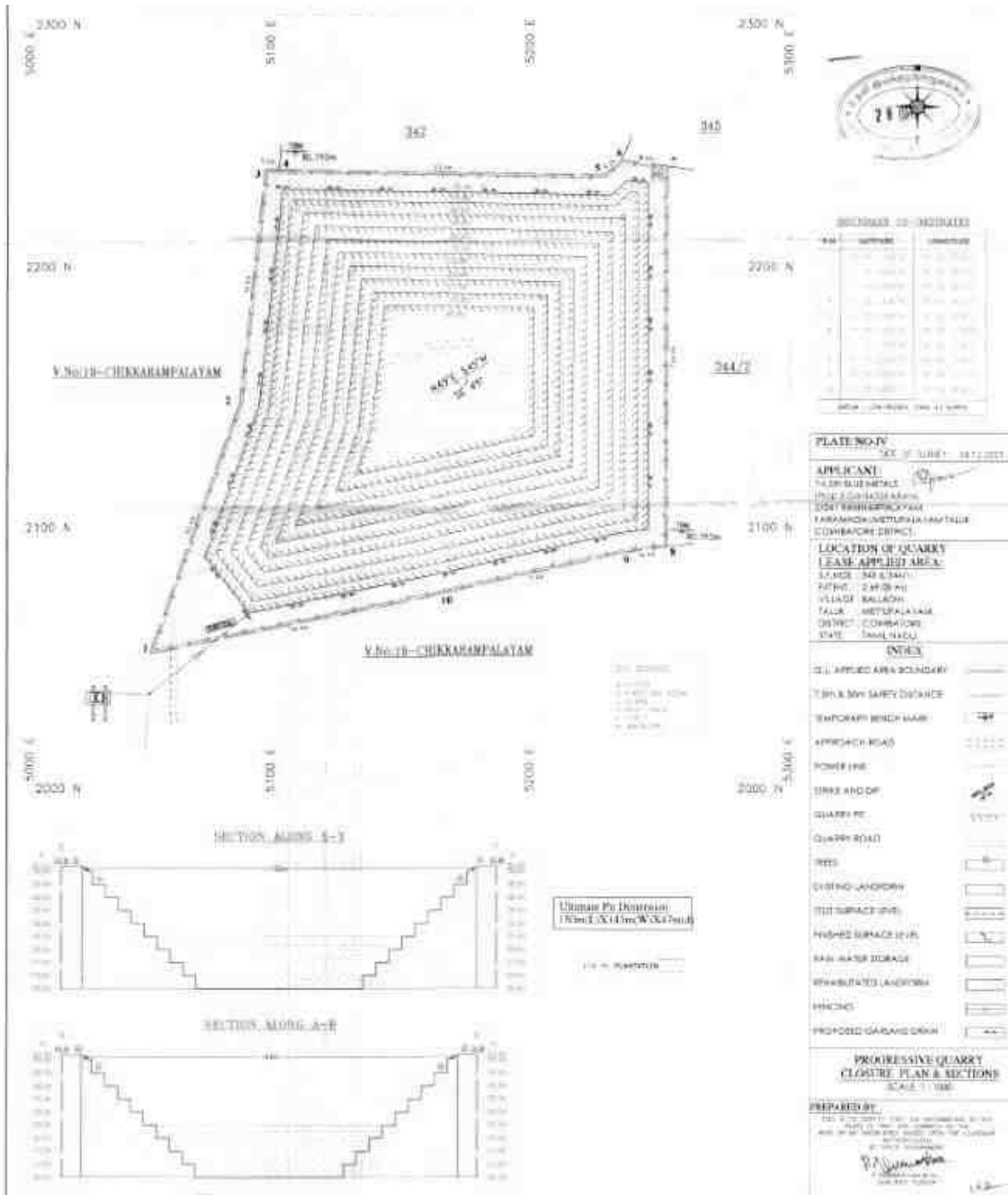
FIGURE 2.24: CLOSURE PLAN AND SECTIONS – P2
