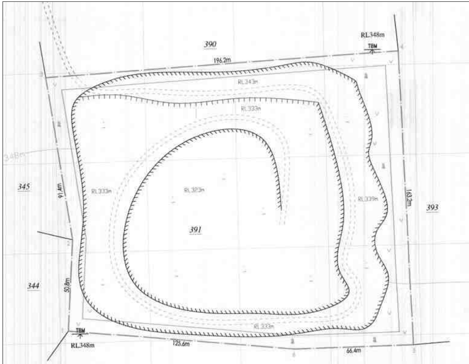
FIGURE 2.9: QUARRY LEASE PLAN / SURFACE PLAN – P3
