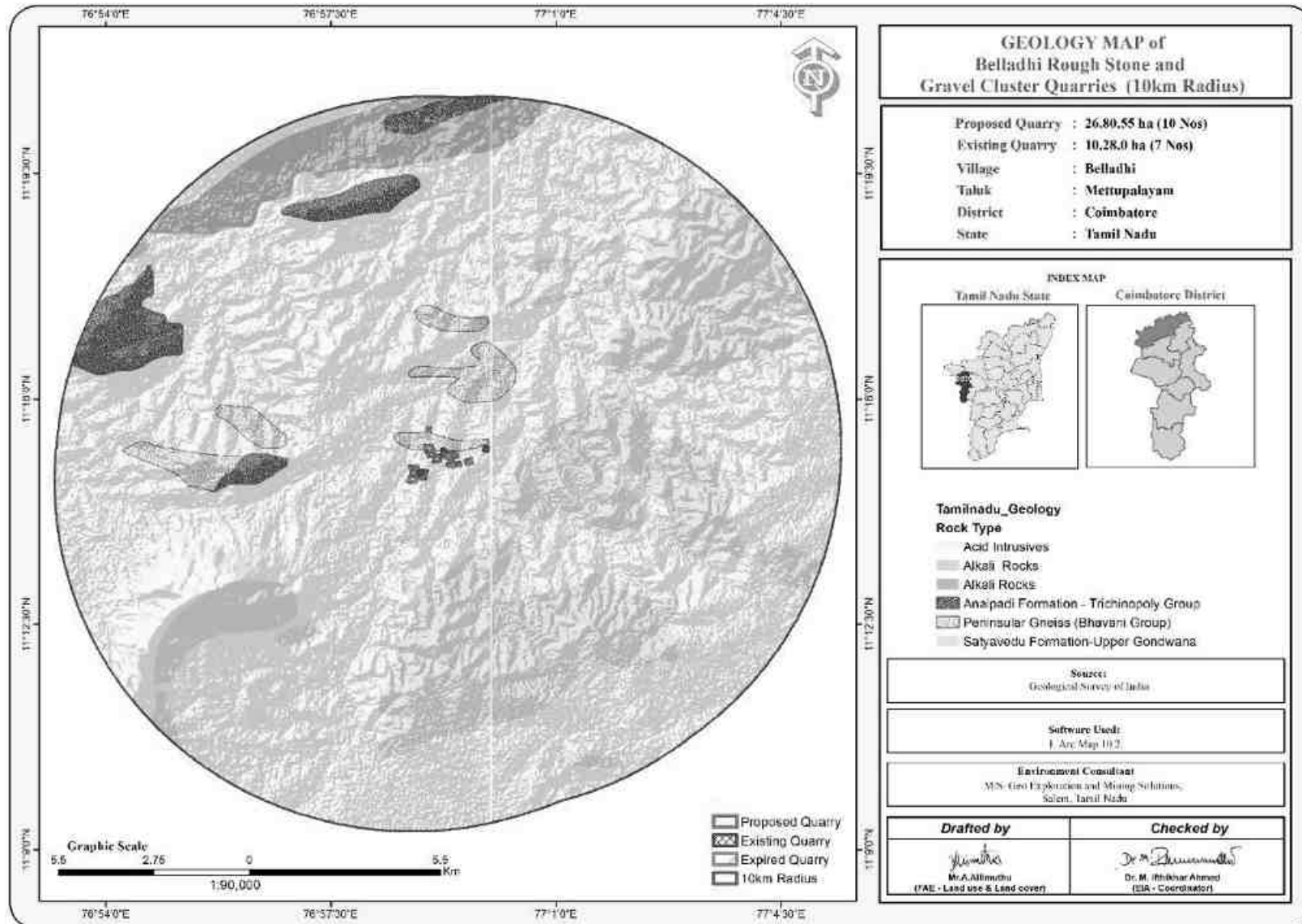
FIGURE 2.15: REGIONAL GEOLOGY MAP
