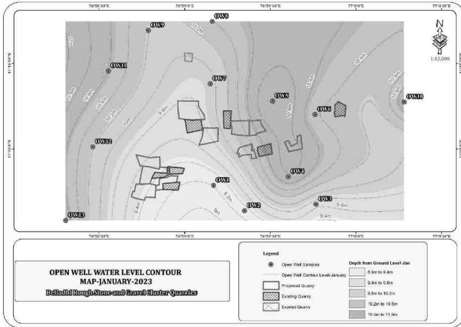
FIGURE 3.7: OPEN WELL CONTOUR MAP – JANUARY 2023
