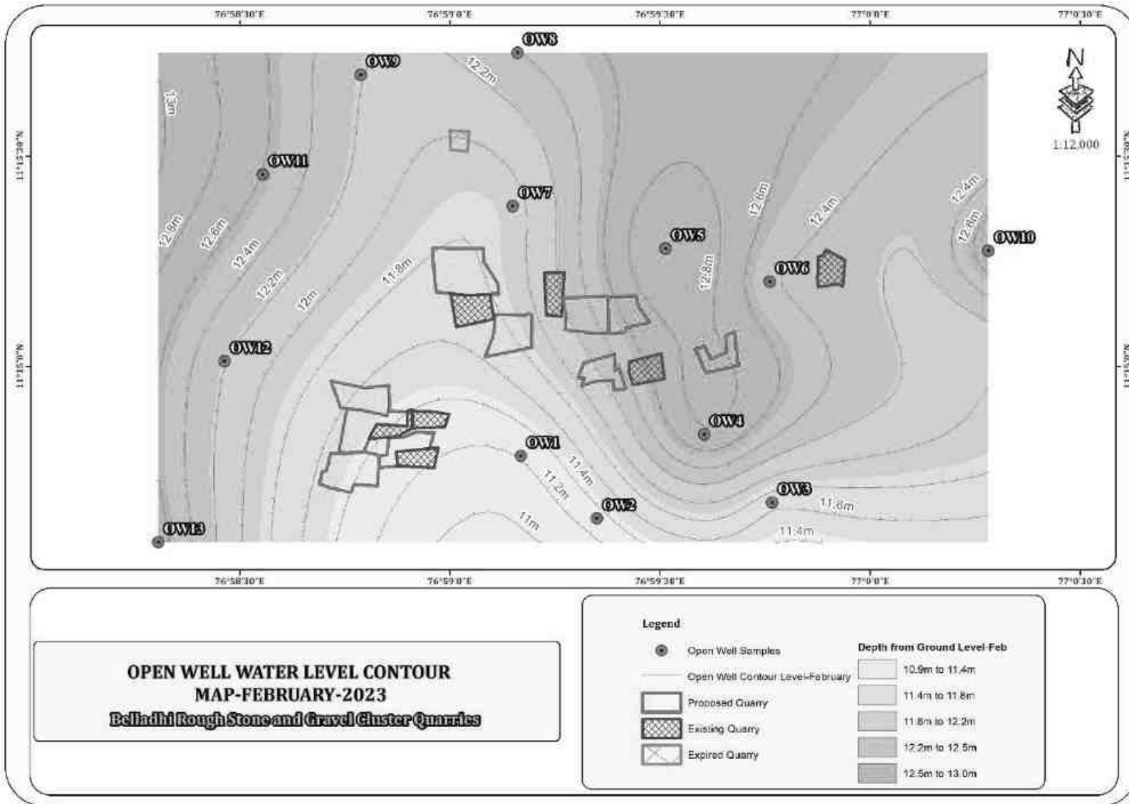
FIGURE 3.8: OPEN WELL CONTOUR MAP – FEBRUARY 2023
