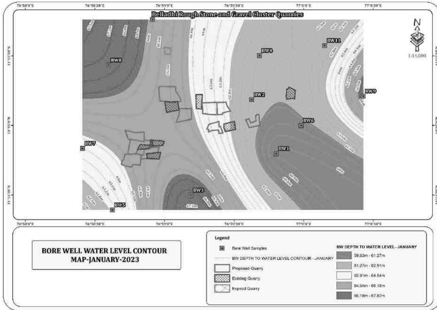
FIGURE 3.10: BOREWELL CONTOUR MAP – JANUARY 2023
