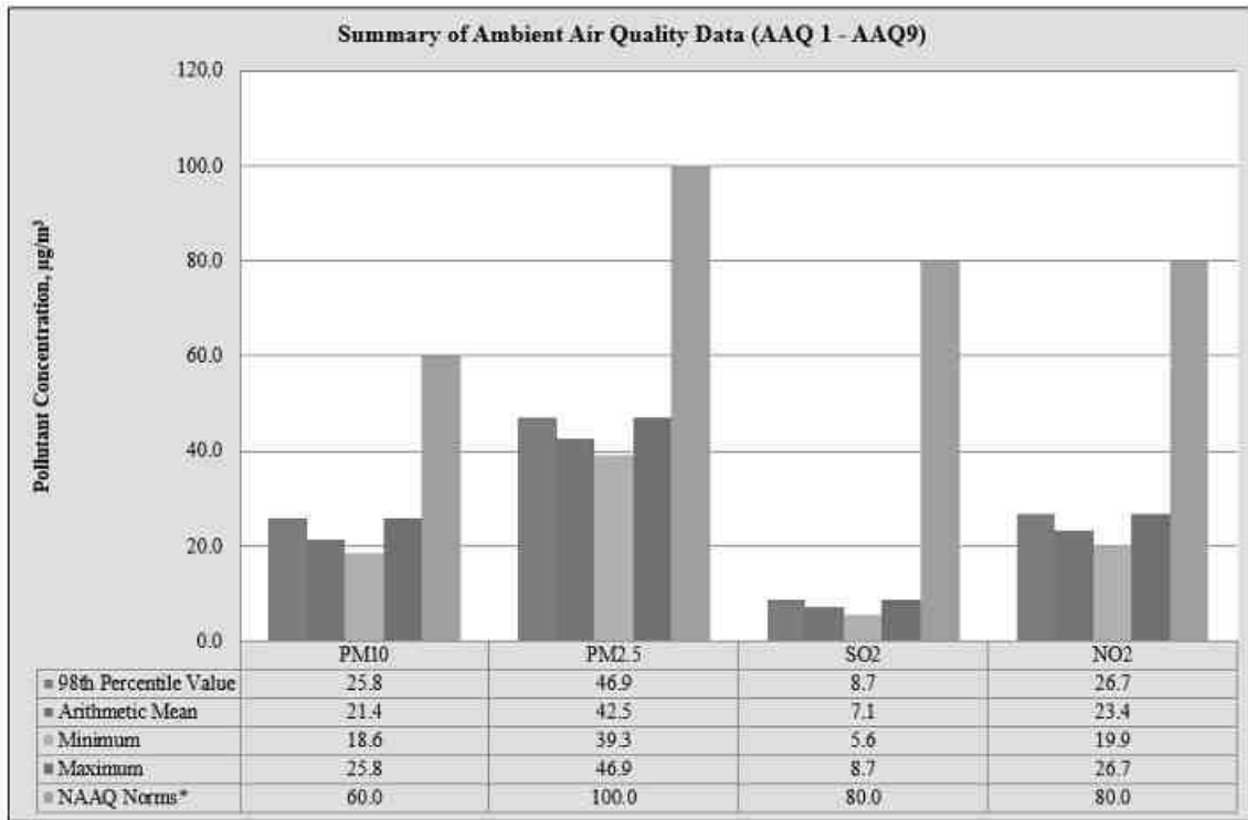
FIGURE 3.16: BAR DIAGRAM OF SUMMARY OF AAQ 1 – AAQ 9
