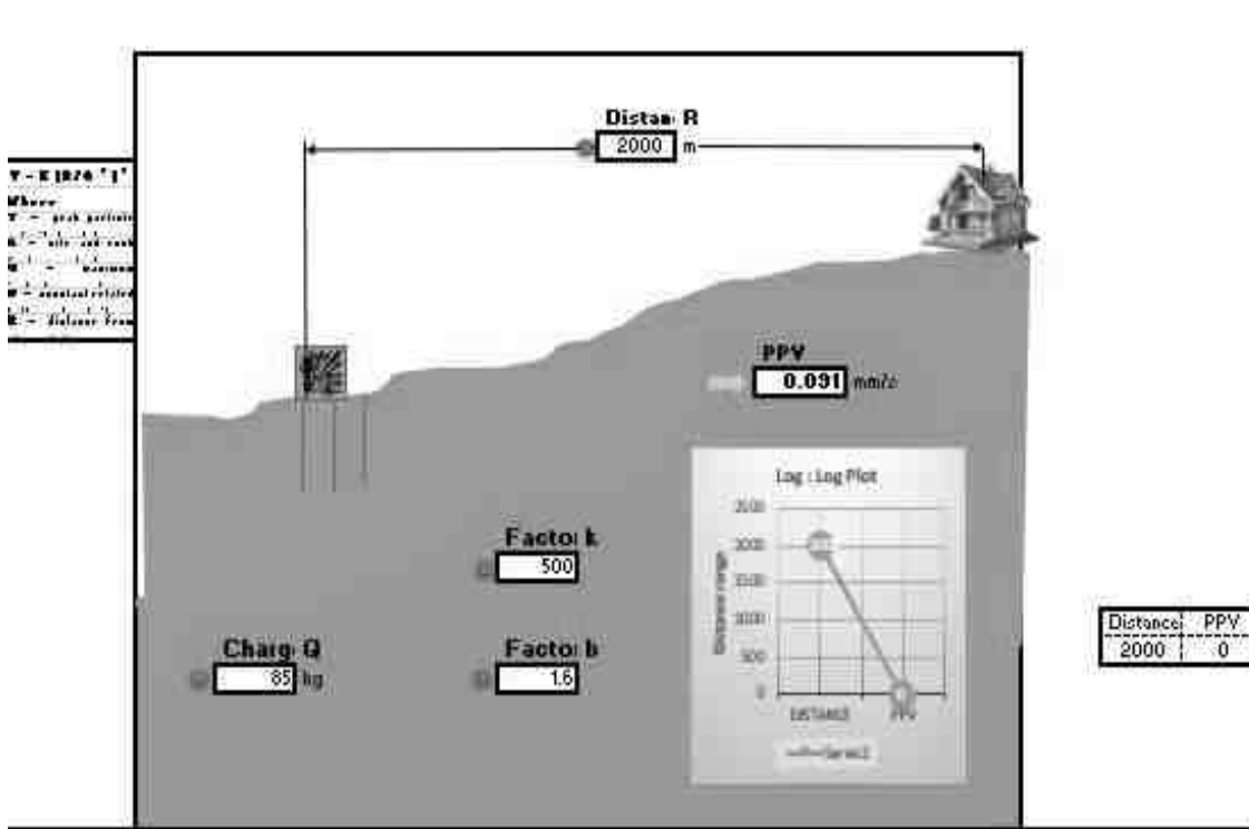
FIGURE 4.6: GROUND VIBRATION PREDICTION
