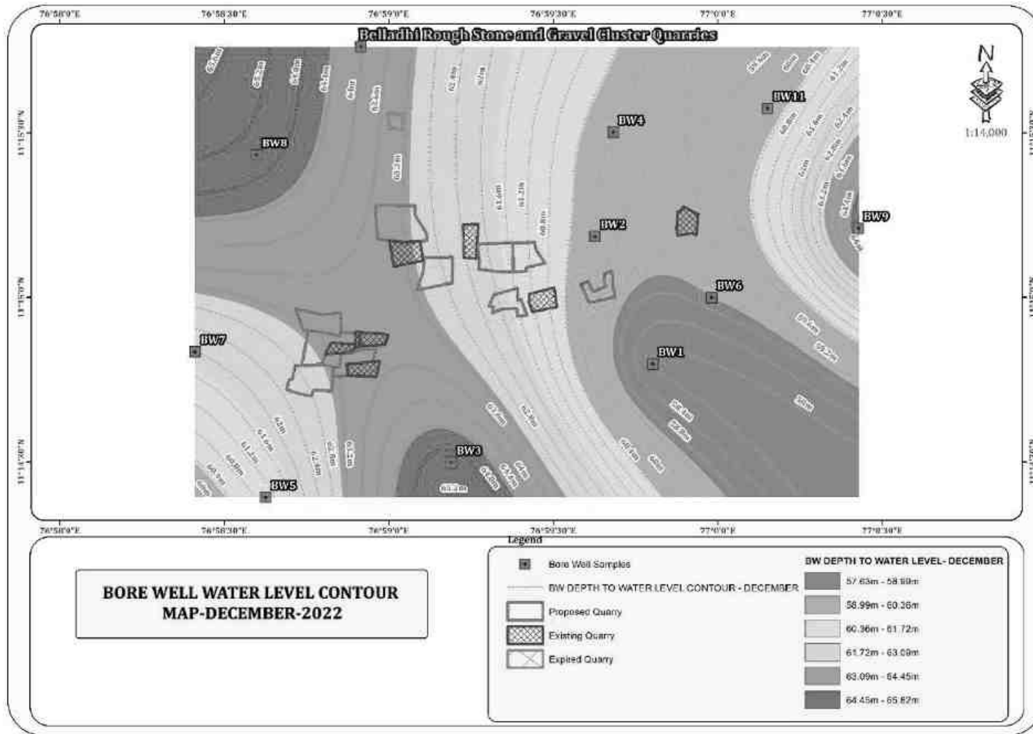
FIGURE 3.9: BOREWELL CONTOUR MAP – DECEMBER 2022
