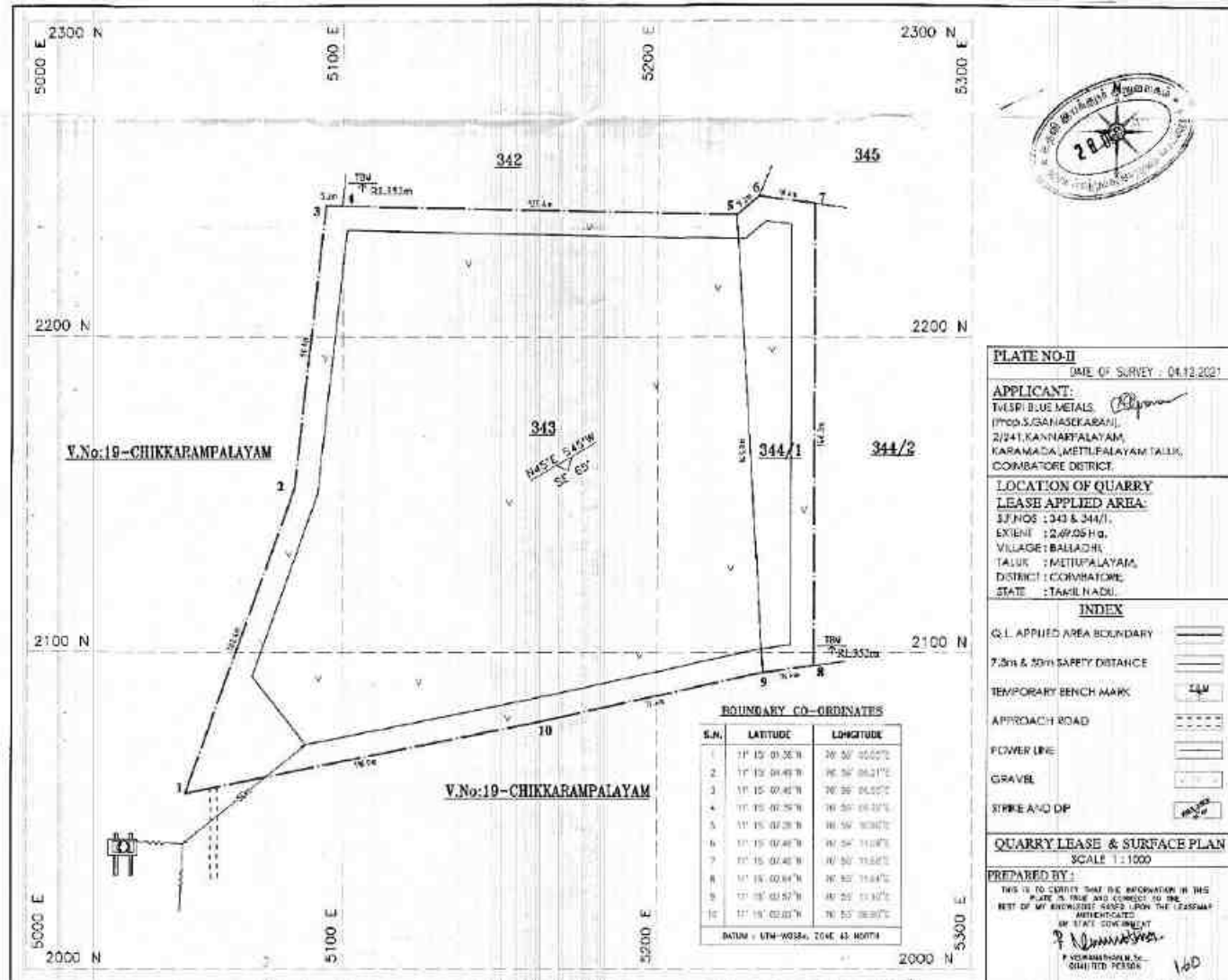
FIGURE 2.8: QUARRY LEASE PLAN / SURFACE PLAN – P2
