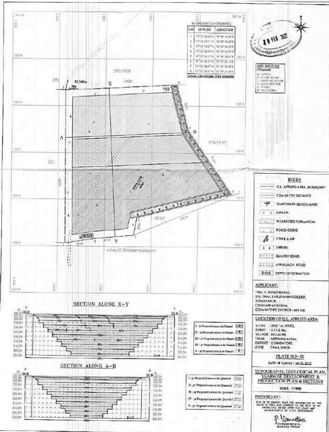
FIGURE 2.17: TOPOGRAPHY, GEOLOGICAL, YEAR-WISE DEVELOPMENT PRODUCTION PLAN AND SECTIONS – P1
