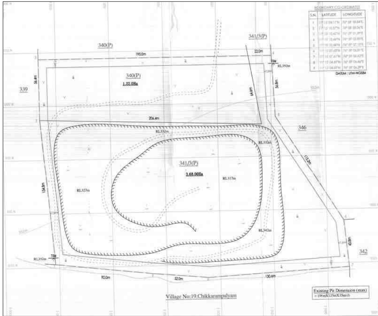
FIGURE 2.10: QUARRY LEASE PLAN / SURFACE PLAN – P4
