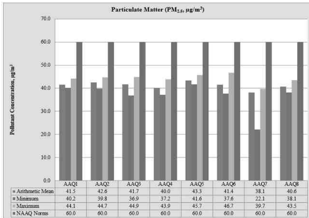
FIGURE 3.17 A : BAR DIAGRAM OF PARTICULATE MATTER (PM 2.5 )
