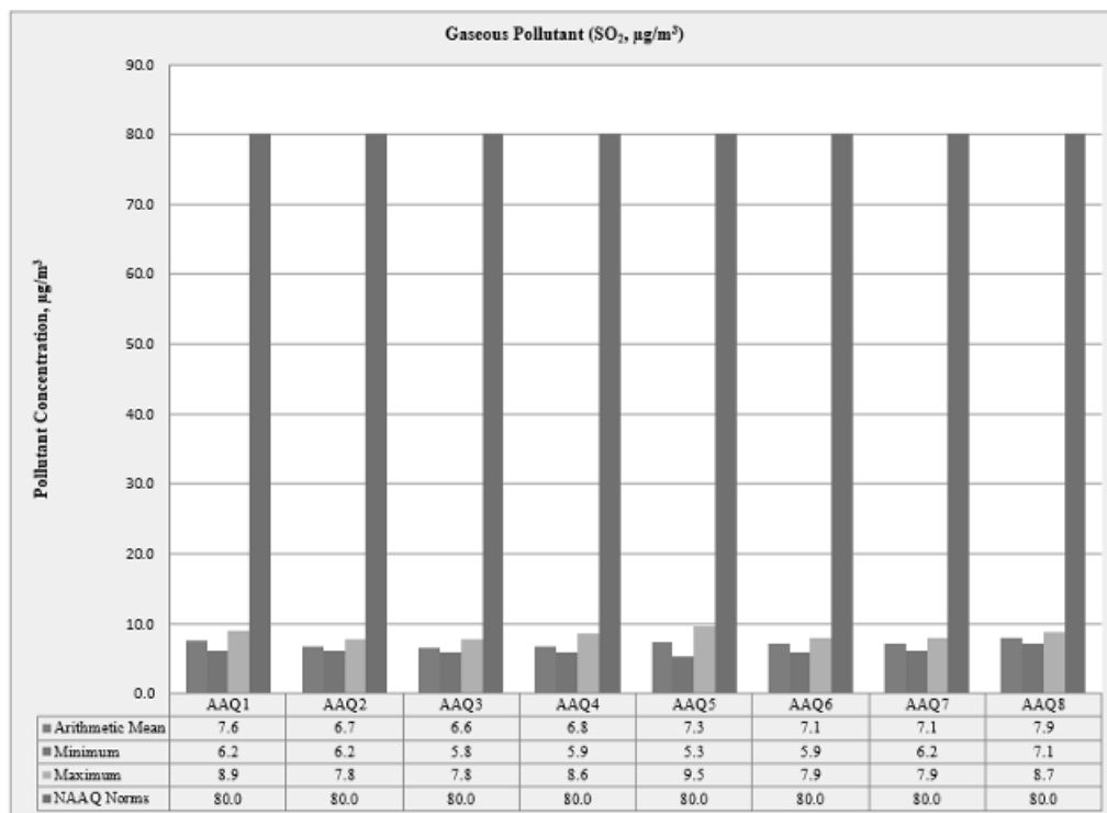
FIGURE 3.17: BAR DIAGRAM OF PARTICULATE MATTER (SO 2 )
