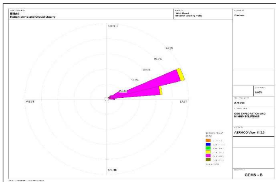
FIGURE – 4: WIND ROSE DIAGRAM
