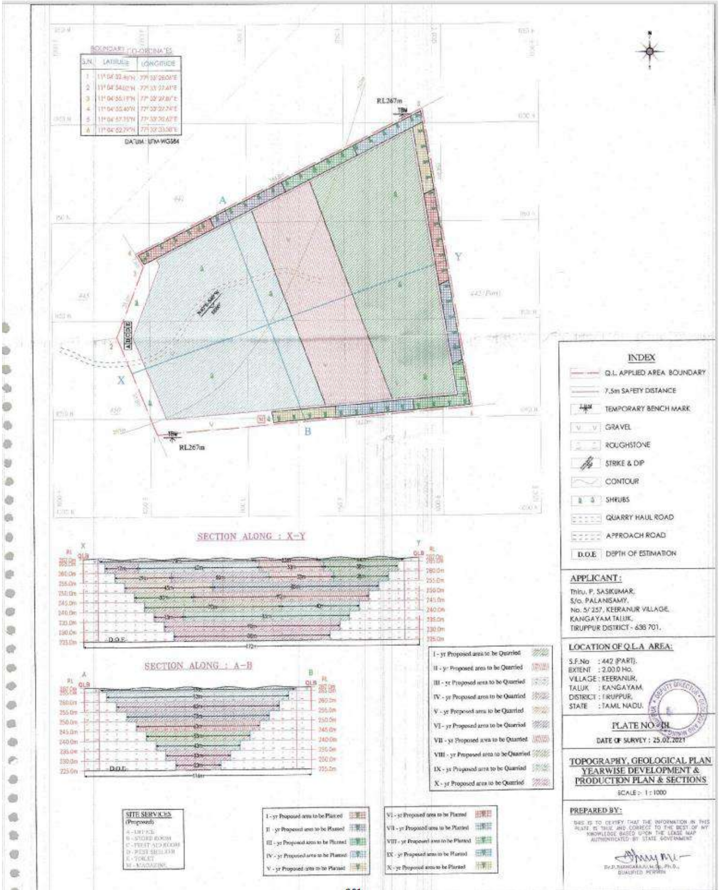
Figure 2.8 Topography, geological plan, year-wise development & production plan and sections
