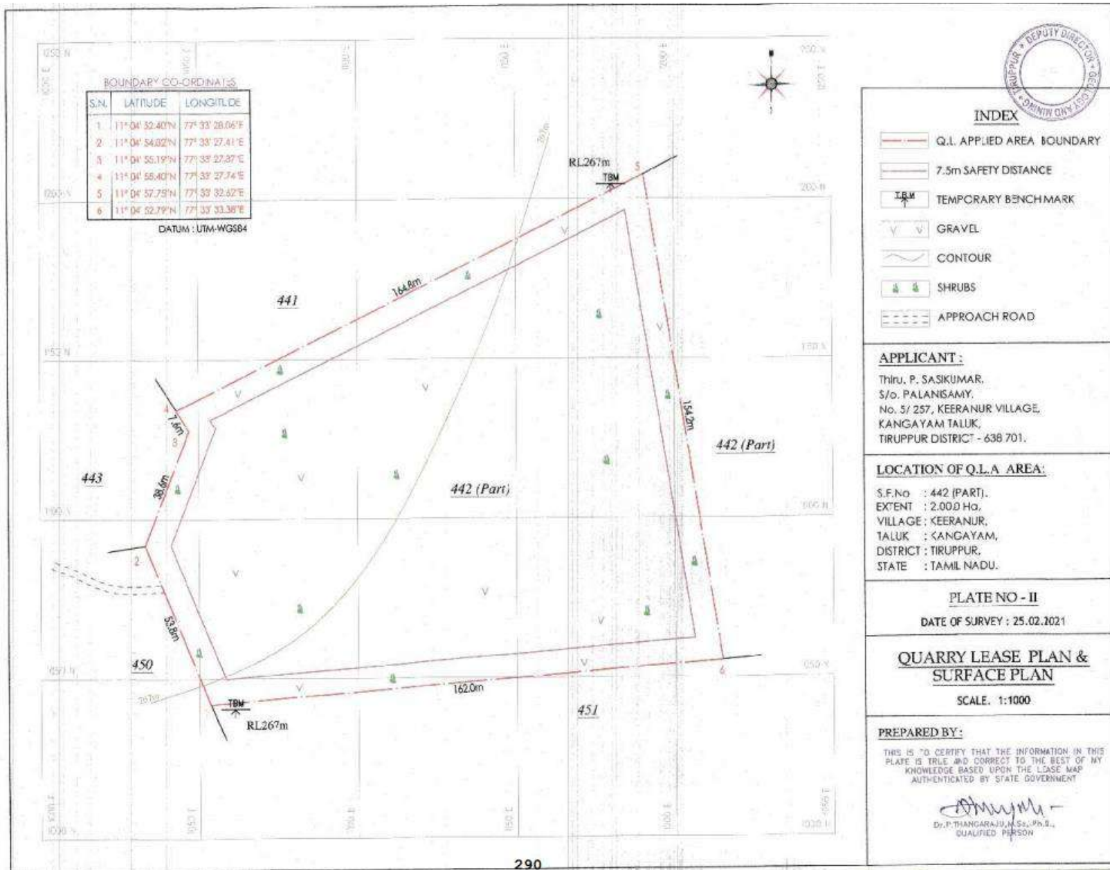
Figure 2.7 Quarry lease plan & surface plan
