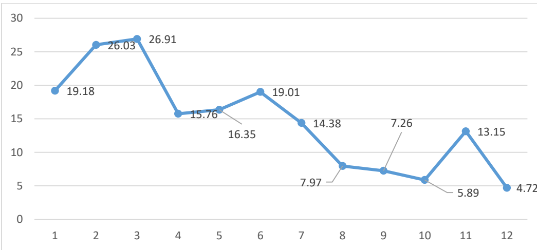
NO 2 ( \mu\text{g}/\text{m}^3 ) Trend Graphs Location: Manali 01-01-2021 to 31-12-2021
