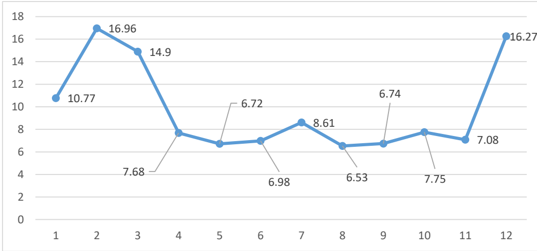
NO ( \mu\text{g}/\text{m}^3 ) Trend Graphs Location: Manali 01-01-2021 to 31-12-2021
