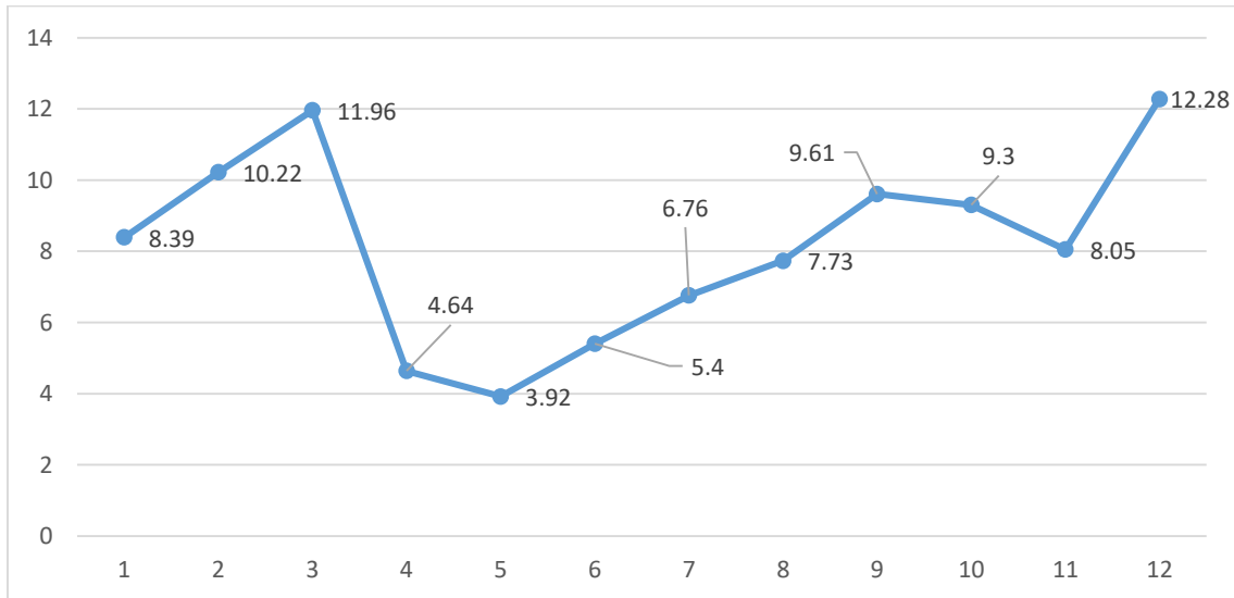
SO 2 ( \mu\text{g}/\text{m}^3 ) Trend Graphs Location: Manali 01-01-2021 to 31-12-2021
