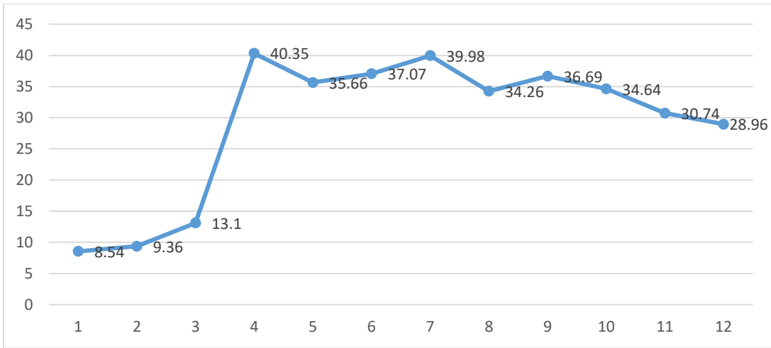
SO 2 ( \mu\text{g}/\text{m}^3 ) Trend Graphs Location: Manali 01-01-2021 to 31-12-2021
