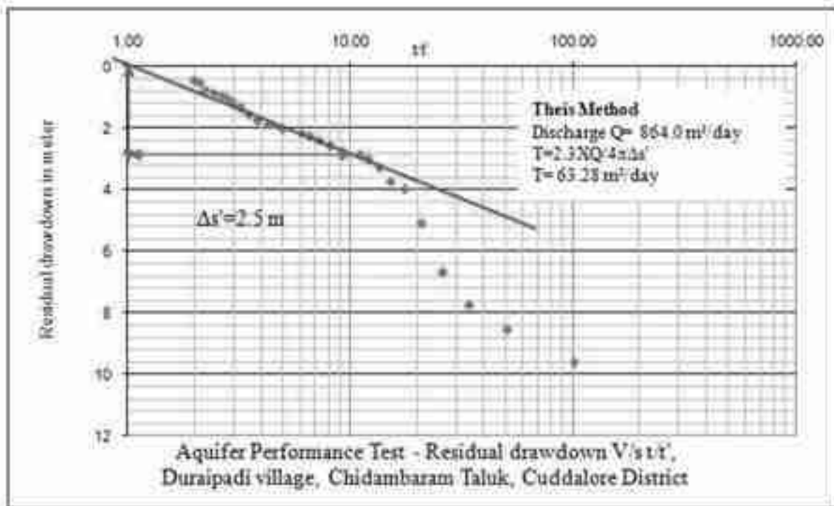
Fig No 3.29 Residual Drawdown Vs t/t' data plot
