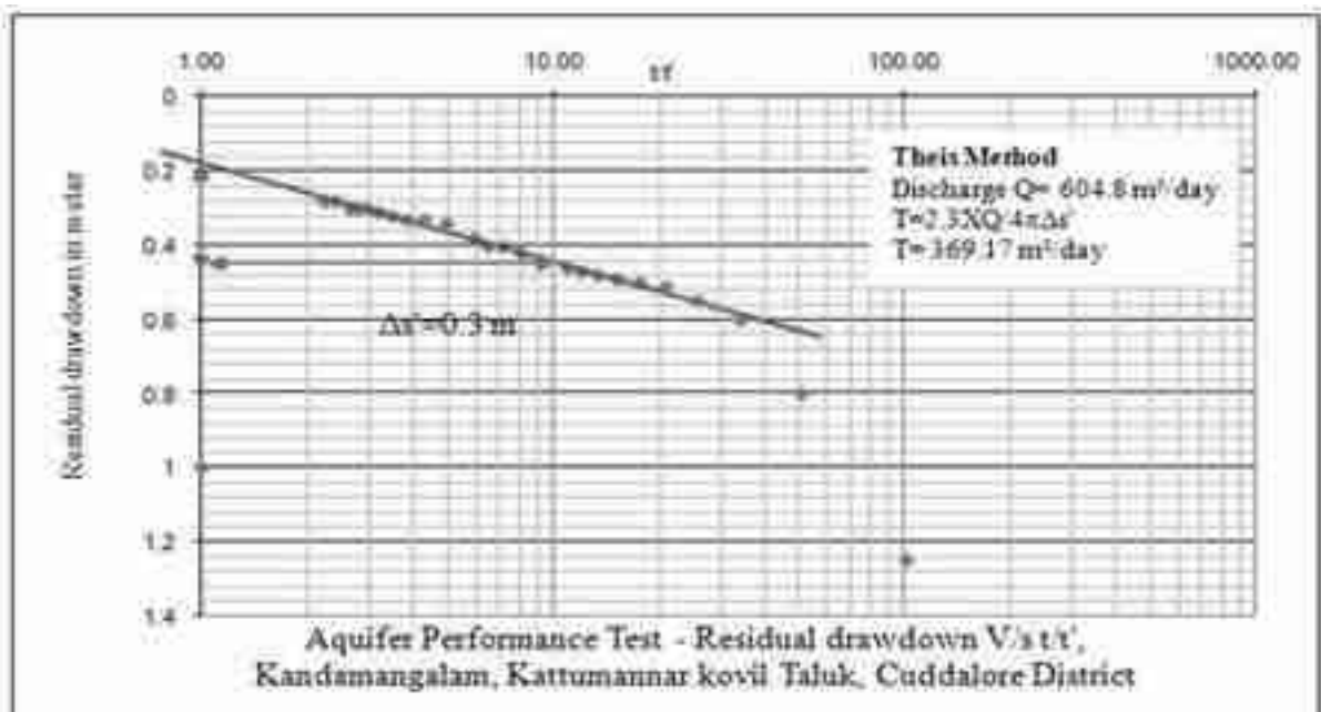
Fig No 3.28 Time V/s Drawdown data plot
