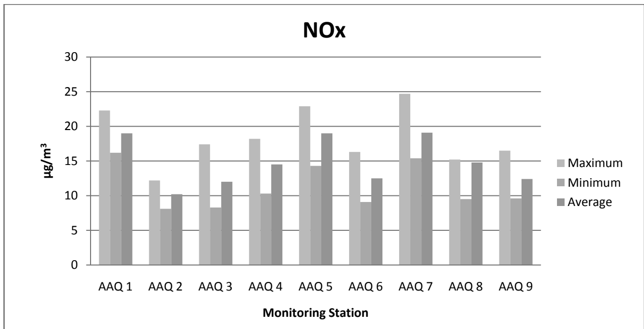
Fig No 3.9: Variation in Concentration of air pollutants during Pre Monsoon Season
