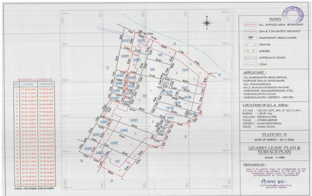
FIGURE – 4: QUARRY LEASE PLAN & SURFACE PLAN
