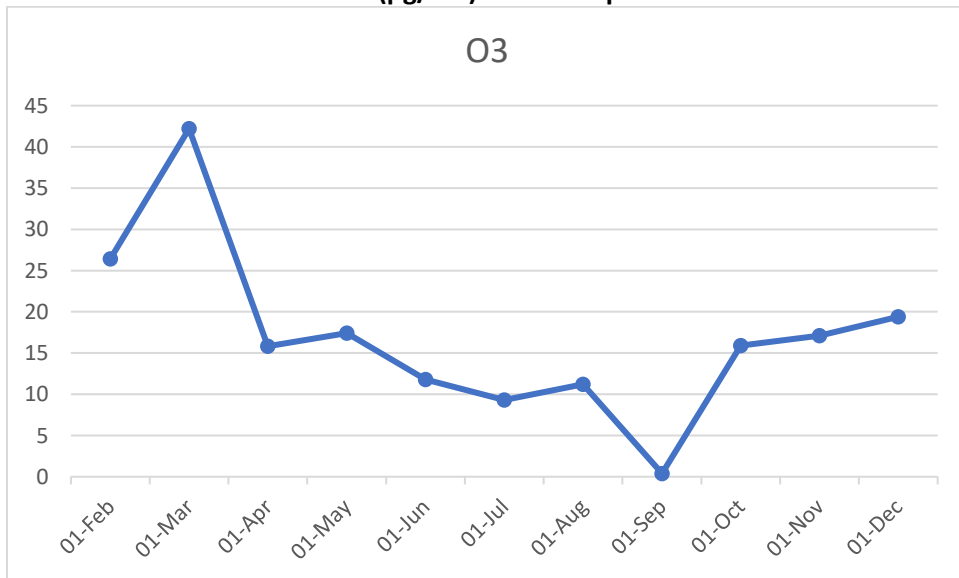
Tamil Nadu Pollution Control Board,CAAQMS O3( \mu\text{g}/\text{m}^3 ) Trend Graph
