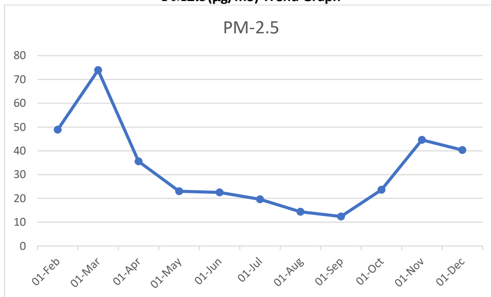
Tamil Nadu Pollution Control Board,CAAQMS PM2.5( \mu\text{g}/\text{m}^3 ) Trend Graph
