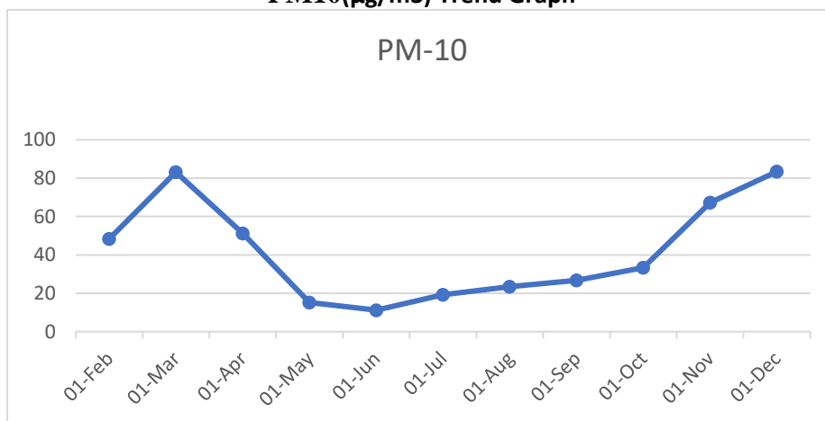
Tamil Nadu Pollution Control Board,CAAQMS PM10( \mu\text{g}/\text{m}^3 ) Trend Graph
