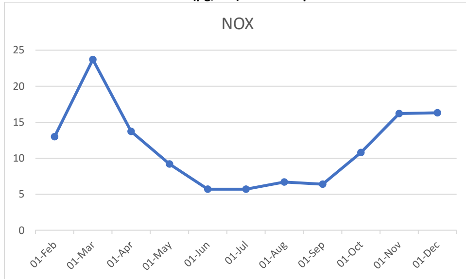
Tamil Nadu Pollution Control Board,CAAQMS NO X ( \mu\text{g}/\text{m}^3 ) Trend Graph
