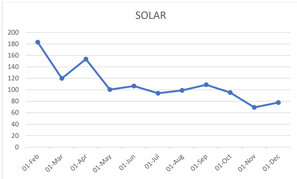
Tamil Nadu Pollution Control Board,CAAQMS SR( \mu\text{g}/\text{m}^3 ) Trend Graph
