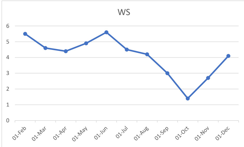
Tamil Nadu Pollution Control Board,CAAQMS WS( \mu\text{g}/\text{m}^3 ) Trend Graph
