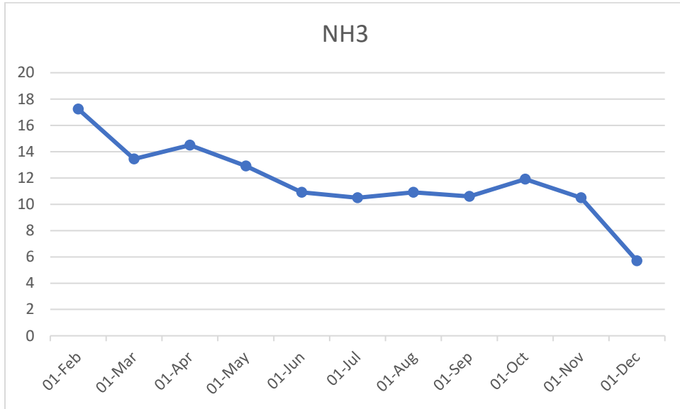
Tamil Nadu Pollution Control Board,CAAQMS NT(μg/m 3 ) Trend Graph
