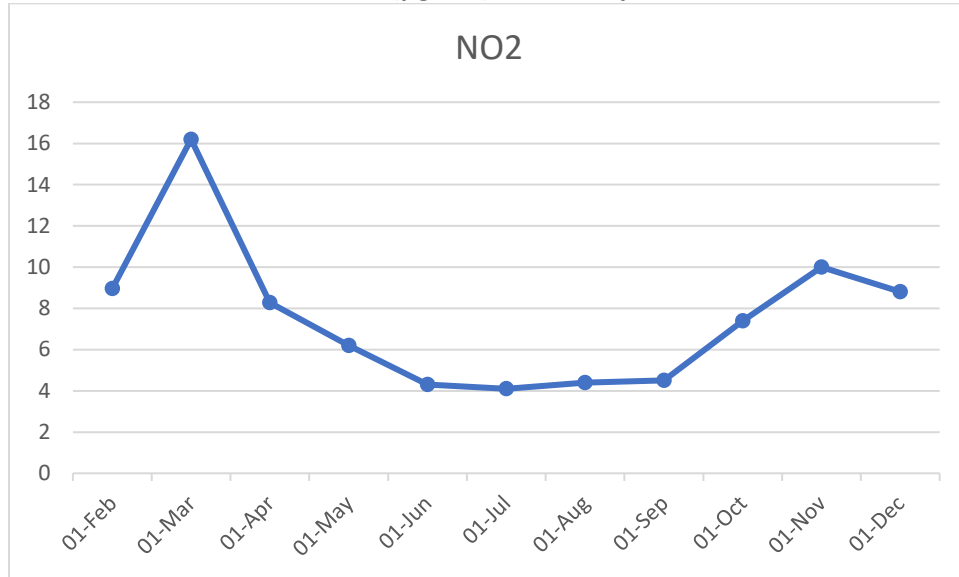
Tamil Nadu Pollution Control Board,CAAQMS NO 2 ( \mu\text{g}/\text{m}^3 ) Trend Graph
