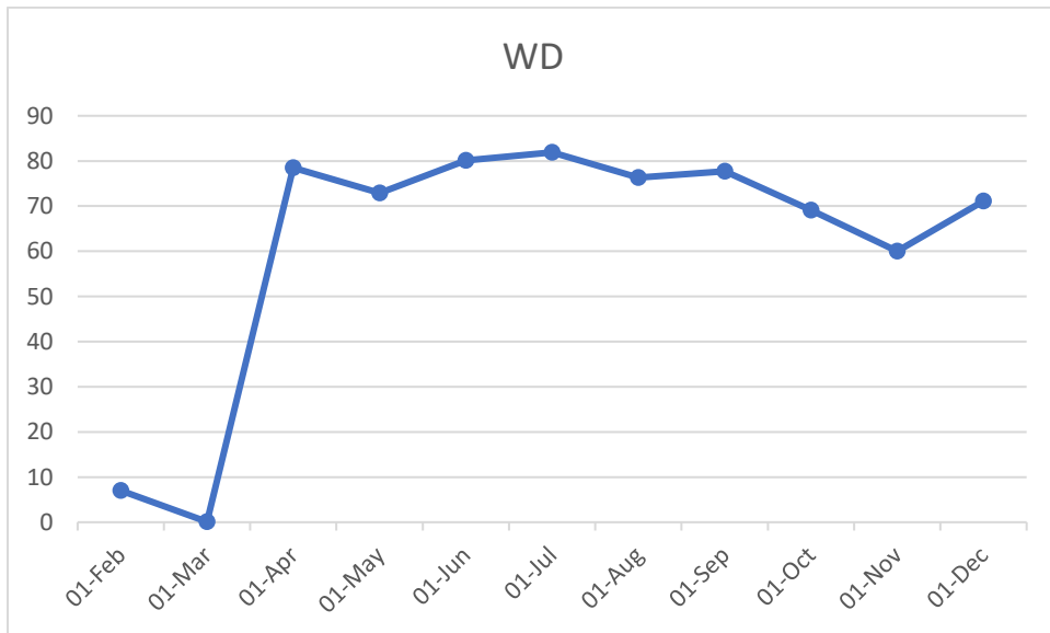
Tamil Nadu Pollution Control Board,CAAQMS WD( \mu\text{g}/\text{m}^3 ) Trend Graph
