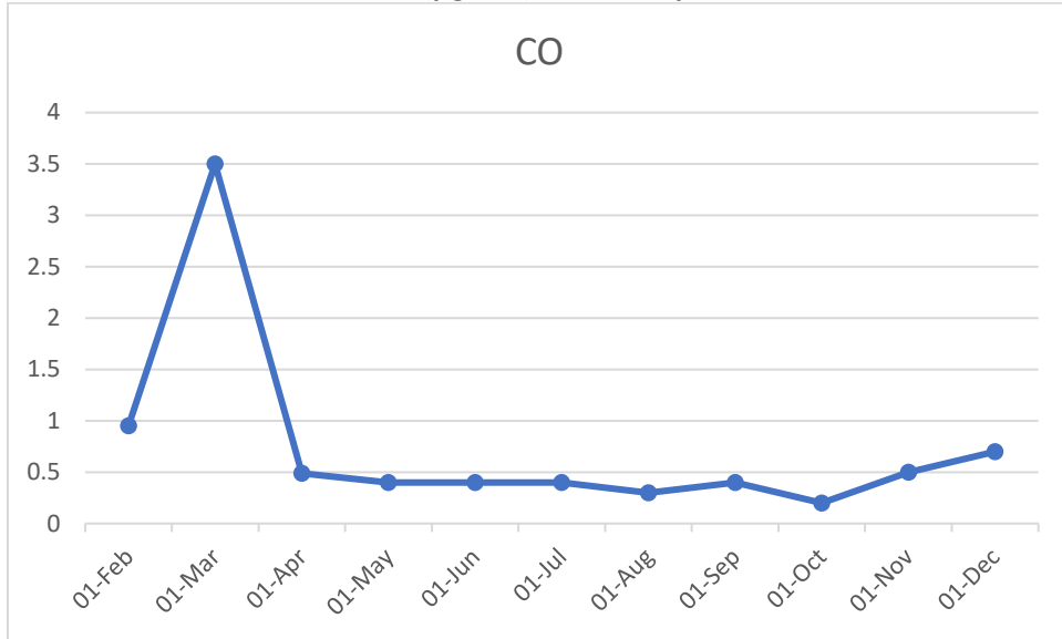
Tamil Nadu Pollution Control Board,CAAQMS CO( \mu\text{g}/\text{m}^3 ) Trend Graph
